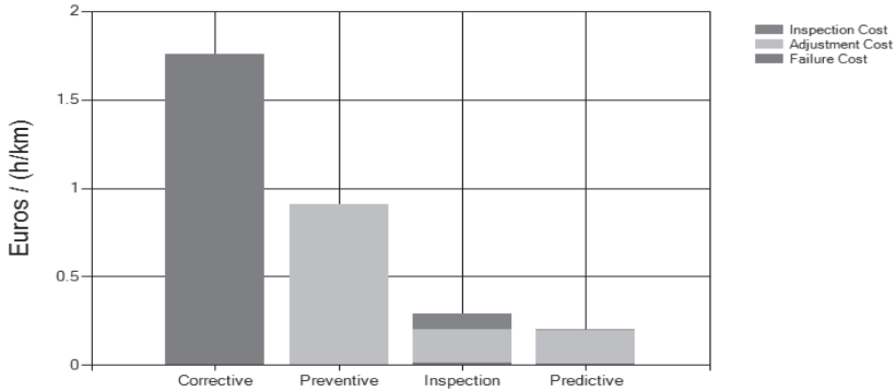
Figure 2. The impact of maintenance strategies segmented by cost categories on mechatronic component.
