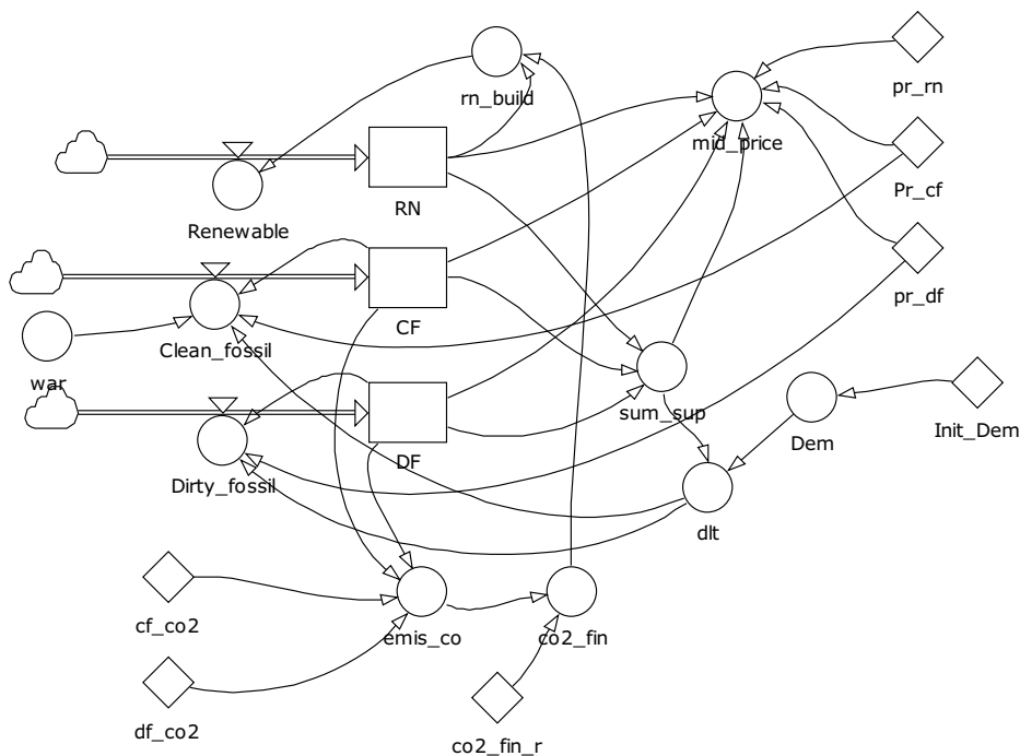
Figure 5. Simulation model of three sectors energy market. Source: [authors' own estimations]
